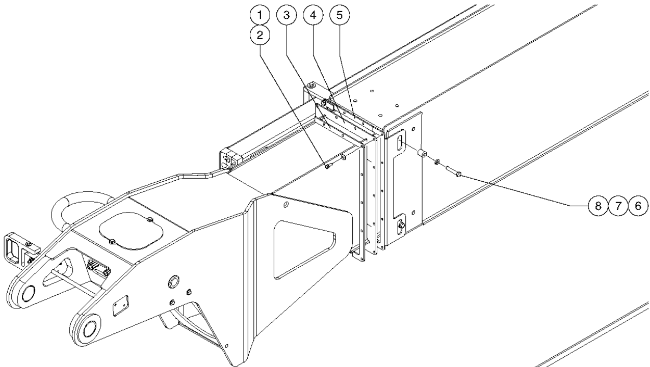
Primary Boom
